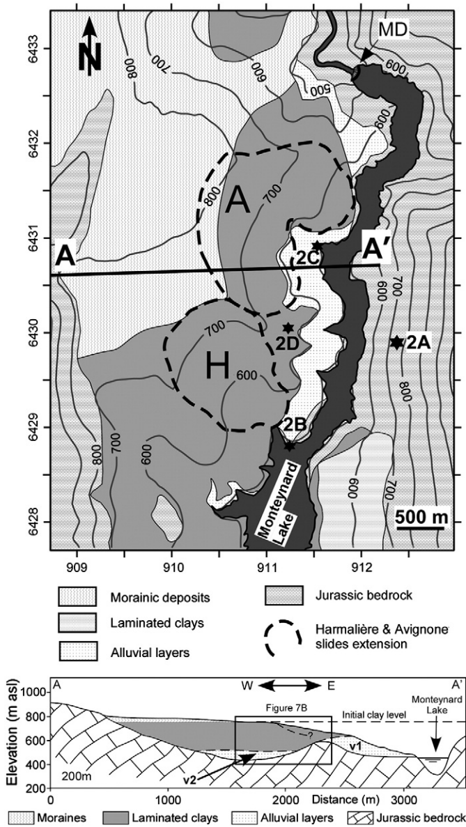
Fig. 3. Geological map (location in Fig. 1) modified from Debelmas (1967) ; Lambert and Montjuvent (1968) and cross section modified after Blanchet (1988) . Black stars refer to pictures in Fig. 2. Position of cross section AA' is indicated. A: Avignonet landslide; H: Harmalière landslide; MD: Monteynard dam. Below: Geological cross section; v1: first paleovalley ("Drac de Cros"); v2: second paleovalley ("Drac de Sinard"). Dashed line within clays depicts the lower limit of the Avignonet landslide, deduced from inclinometer data. See text for details.
