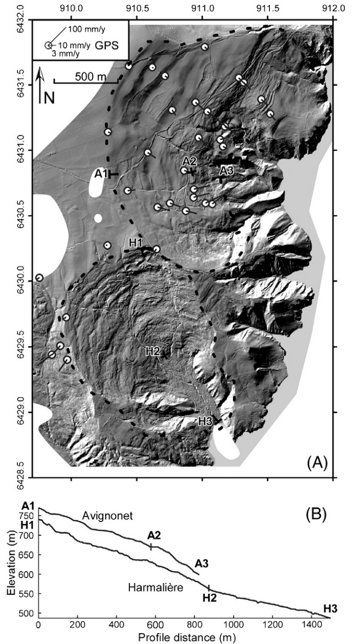
Fig. 4. (A) Shaded LiDAR DEM (light direction is from NW, horizontal resolution of 2 m) covering the Avignonet (north) and Harmalière (south) landslides. Dotted lines indicate the landslide limits. The white circles show the position of the GPS points, and the thin straight lines represent the 11-year average horizontal velocity measured by GPS. A1–3 and H1–3 indicate the location of the elevation profiles. (B) Elevation profiles through Avignonet and Harmalière with subdivisions in an upper and lower part. Profiles are 2× vertically exaggerated.
