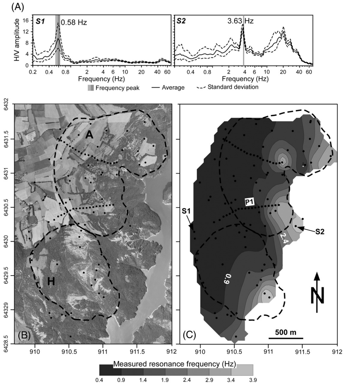
Fig. 6. H/V measurements. (A) H/V curves at points S1 and S2 (location on Fig. 6C). (B) Location of the 104 measurement points with the landslide limits (dashed line); A: Avignonnet landslide; H: Harmalière landslide. (C) Resonance frequency map.
