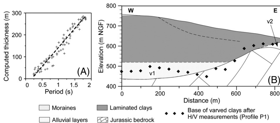
Fig. 7. Frequency to thickness calibration for H/V profile P1 (location on Fig. 5B and C). (A) Computed thickness as a function of the measured resonance period (inverse of the frequency) for the 104 stations. Linear regression (black dashed line) gives a determination coefficient r^2 of 0.95; (B) Comparison of the geometry of the top of the Jurassic bedrock (Blanchet, 1988) and the bottom of the laminated clays after H/V measurements along profile P1 (location in Fig. 6C). Dashed line depicts the lower limit of the Avignonet landslide deduced from inclinometer data.
