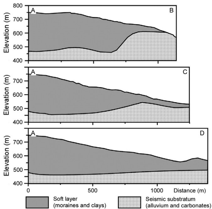
Fig. 9. Cross sections of the paleolake basement (location in Fig. 8B).
