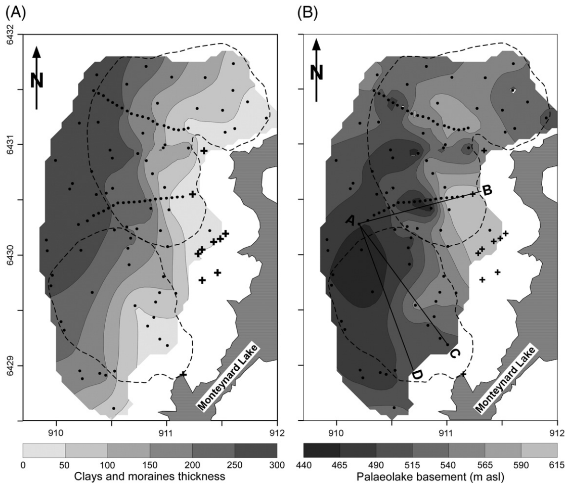
Fig. 8. (A) Thickness maps of the lacustrine deposits. The absolute error between computed and interpolated thicknesses is 5.29%. (B) Lake Trièves paleotopography in the study area. The absolute error between computed and interpolated paleotopography is 0.98%. Dots refer to seismic measurements and crosses to field observations; dashed lines stand for Avignonet and Harmalière landslide limits.
